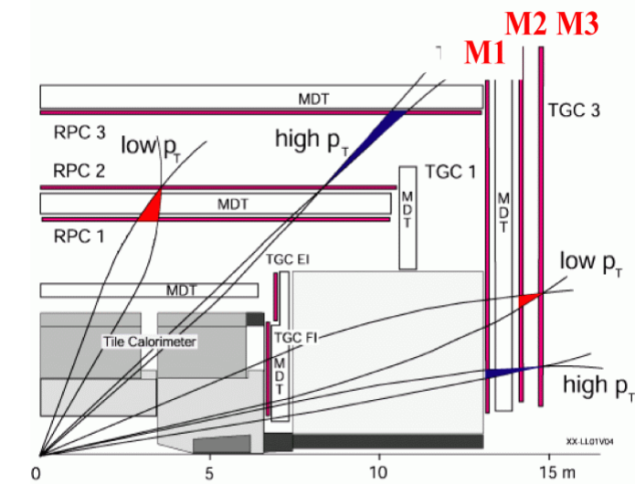
Figure 1: ATLAS Muon Level 1 Trigger Scheme
