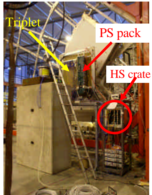
Figure 4: On detector electronics setup around the triplet
