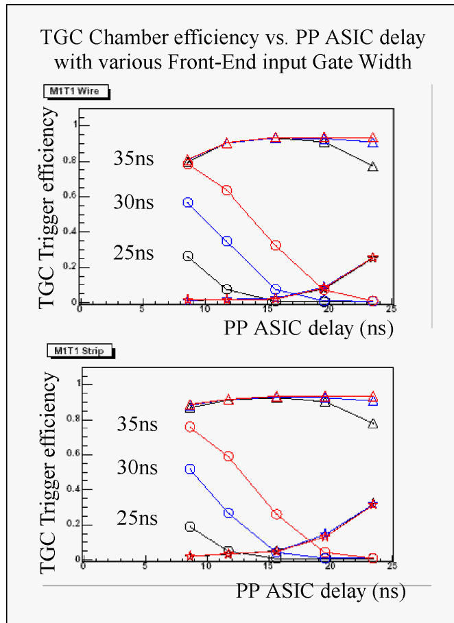
Figure 5: Chamber efficiency for the 1 st one of the triplet versus PP ASIC delay adjustment with three different gate widths (25, 30 and 35ns). Triangle shows data recognized as the right bunch, and the circle (star) represents data in the previous (next) bunch.
