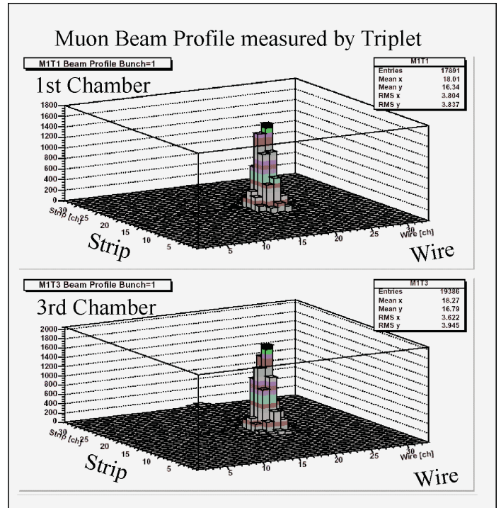
Figure 6: Two dimensional Beam profile measured by the first and third chambers of the triplet.
