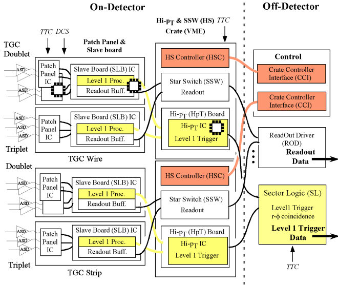
Figure 1: Figure 3: Overview of TGC electronics
