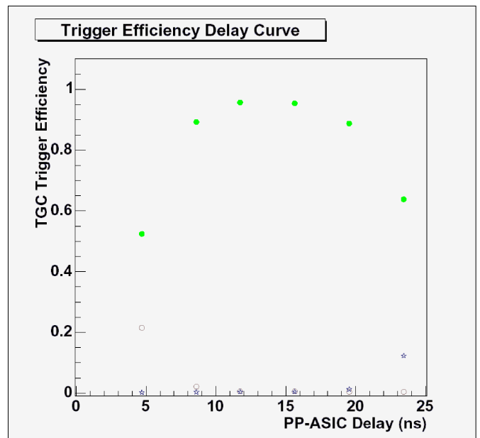
Figure 7: Trigger efficiency versus delay value set of PPASIC
